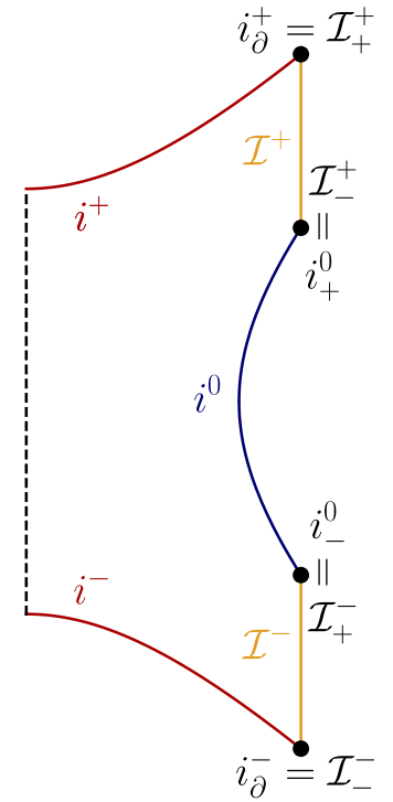
Figure 6.2: Overlap regions
