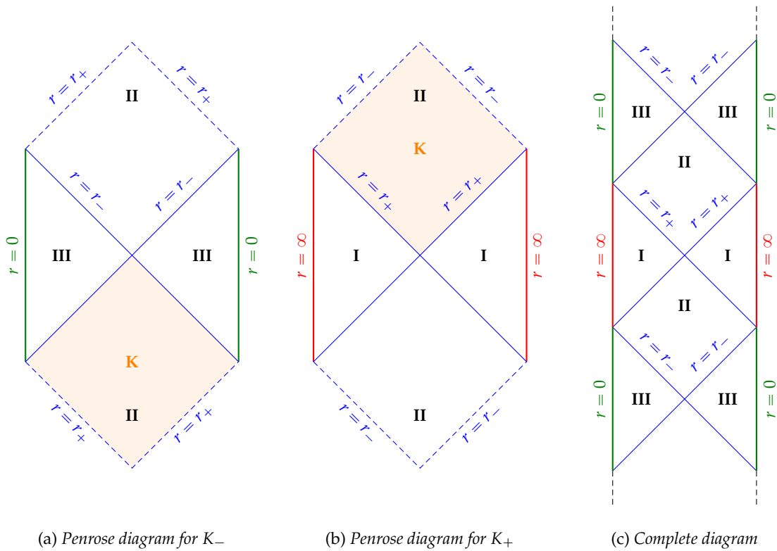
Figure 1.3: Penrose diagrams for non-extremal BTZ black holes
