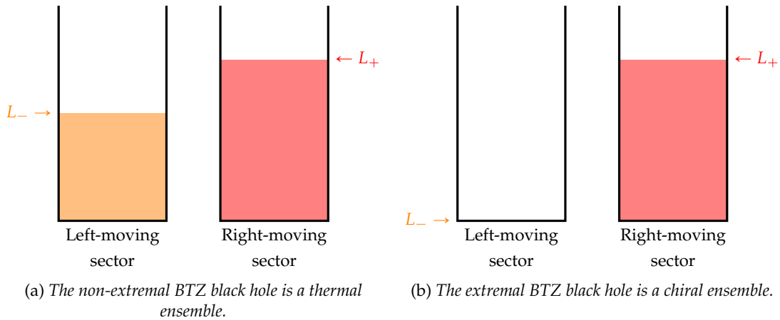
Figure 5.5: CFT thermal and zero temperature ensembles associated to the BTZ black hole.
