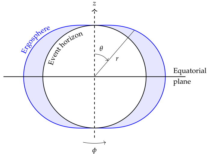
Figure 5.1: Ergoregion of the Kerr black hole ( t fixed).
