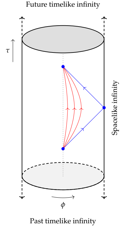
Figure 1.1: Penrose diagram of global AdS_3 spacetime.
