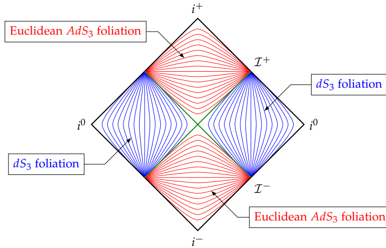
Figure 6.3: Hyperbolic foliations which blow up the geometry near the singular points i^+, i^-, i^0 . The origin lightcone (centered at r = t = 0 ) is drawn in green.
