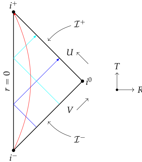
Figure 2.1: Penrose conformal diagram of Minkowski spacetime \mathbb{R}^{(2,1)} . Radial null geodesics are represented in blue, while a radial timelike geodesic is represented in red.
