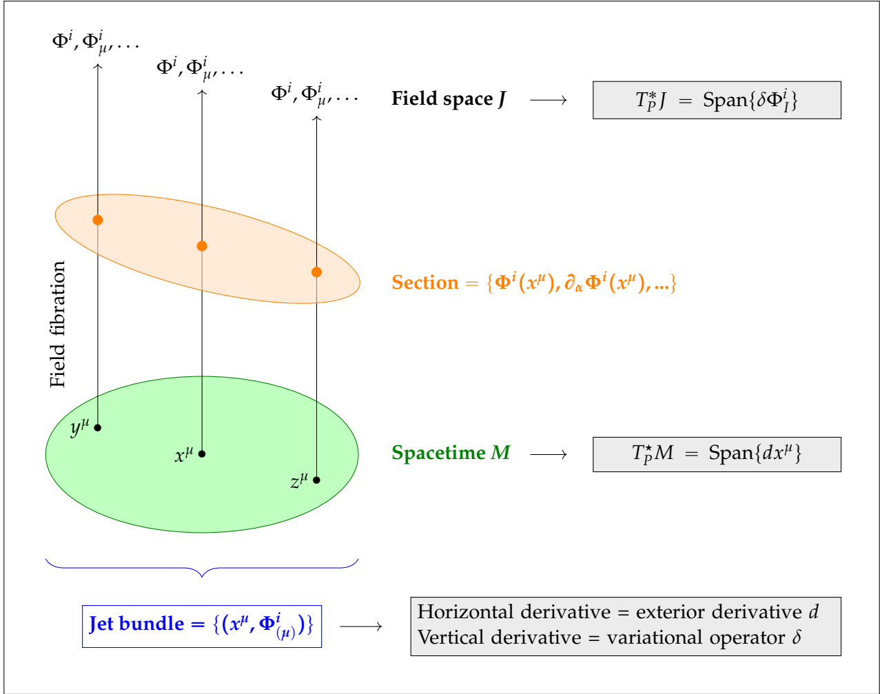
Figure 3.1: Elements from the variational bicomplex structure.
