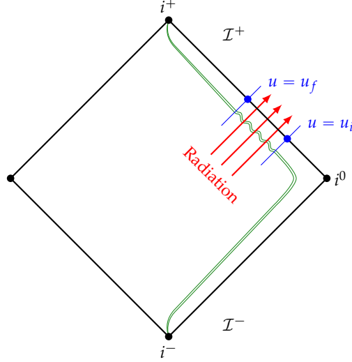
Figure 6.6: Displacement memory effect.
