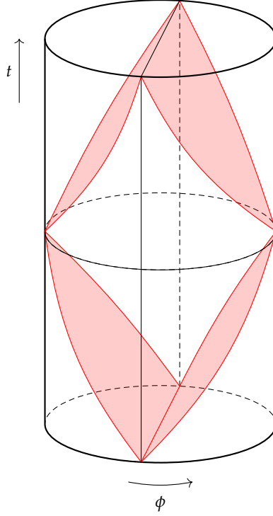
Figure 1.6: A finite-time section of the conformal representation of AdS_3 . The red sections are the null surfaces on which \zeta^2 = 0 .
