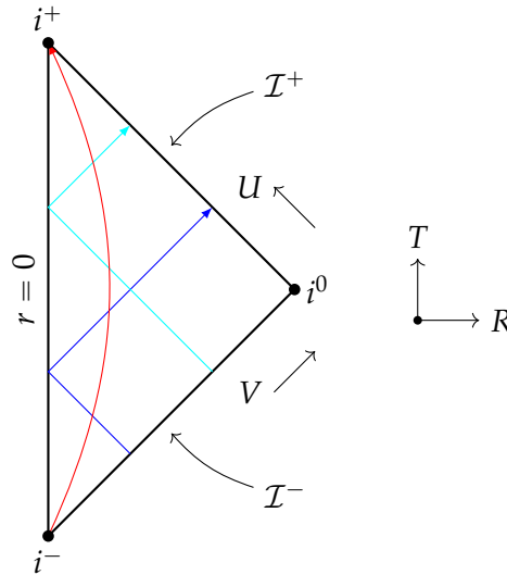
Figure 6.1: Penrose conformal diagram of Minkowski spacetime \mathbb{R}^{(3,1)} . Radial null geodesics are represented in blue, while a radial timelike geodesic is represented in red.
