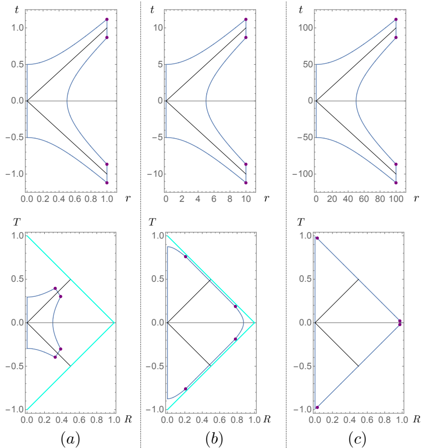
Figure 6.4: The five infinities can be represented as the boundaries of the region defined by |t^2 - r^2| < \mathcal{T} and r < \mathcal{R} for large constants \mathcal{T} and \mathcal{R} . This boundary is plotted for a sequence (a) \mathcal{T} = 0.25, \mathcal{R} = 1 ; (b) \mathcal{T} = 25 and \mathcal{R} = 10 ; and (c) \mathcal{T} = 2500 and \mathcal{R} = 100 , showing the 4 overlapping boundary regions as bullets. The “puzzle piece” shape is invariant on a Minkowski spacetime diagram (top), but converges to a diamond on a conformal diagram (bottom). The puzzle piece adequately represents all asymptotic regions, while the conformal diagram does not resolve i^+, i^- and i^0 , nor any of the overlap regions.
