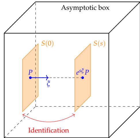
Figure 1.5: Identifications in AdS_3 .
