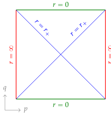
Figure 1.2: Penrose diagram for a static BTZ black hole ( J = 0 ).
