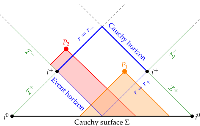
Figure 5.3: The inner horizon is a Cauchy horizon.
