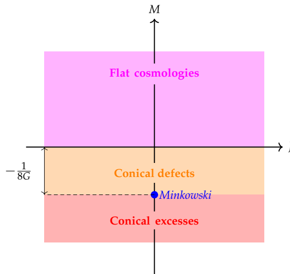
Figure 2.2: Constant representatives of the asymptotically flat phase space.
