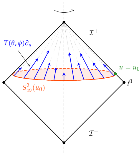
Figure 6.5: BMS supertranslations
