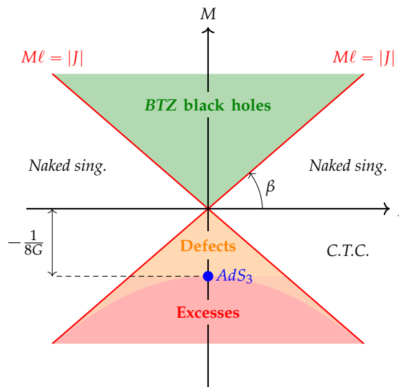
Figure 1.7: Solutions described by the BTZ metric.
